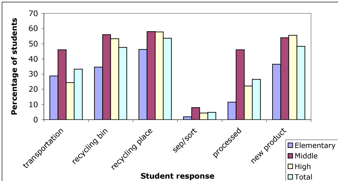
Figure 8. Percentage of elementary, middle, and high school students who mentioned steps of paper cup recycling waste disposal chain
