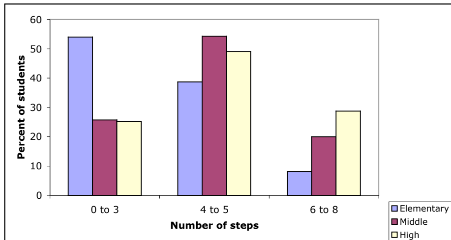
Figure 3. Number of steps mentioned by elementary, middle, and high school students for the hamburger supply chain.
