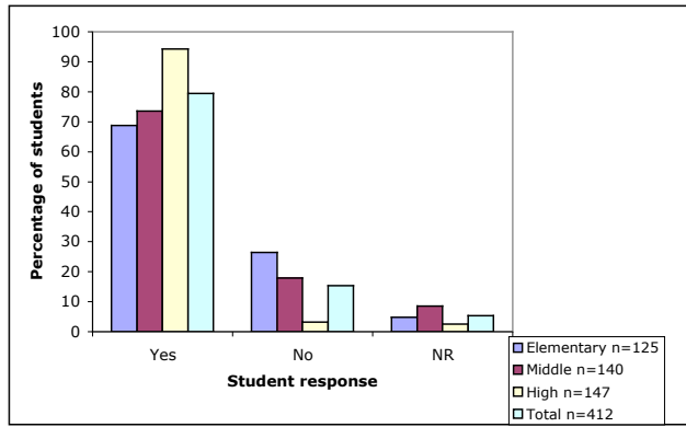
Figure 10a. Percentage of elementary, middle and high school student responses to awareness of global warming.
